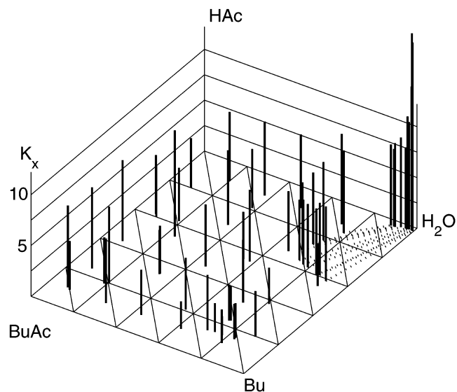
Figure 7. Experimental pseudoreaction equilibrium constant in the system water + 1-butyl acetate + 1-butanol + acetic acid at 373.15 K: —, experimental K_x ; ·····, experimental conodes.
