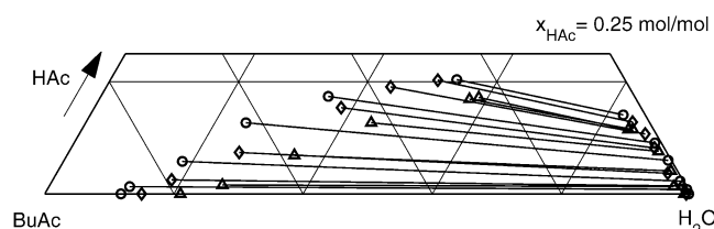
Figure 4. Liquid–liquid equilibria in the pseudoternary system water + 1-butyl acetate + acetic acid: ○, 353.15 K; ◇, 373.15 K; △, 393.15 K.
