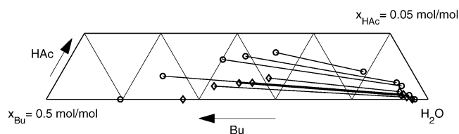
Figure 5. Liquid–liquid equilibria in the pseudoternary system water + 1-butanol + acetic acid: ○, 353.15 K; ◇, 373.15 K.
