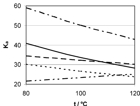
Figure 12. Comparison between K_a calculated from the Gibbs free energy of reaction to K_a fitted to the experimental data of the present work. Models: —, Gibbs free energy of reaction; ·····, NRTL; - - -, UNIQUAC; - · -, PC-SAFT; - - - -, COSMO-RS.
