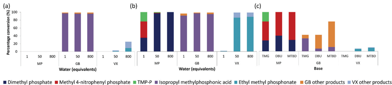
Fig. 4 Testing of 1, 50, and 800 equivalents of water, with respect to the simulant MP and CWAs GB and VX, in (a) the absence and (b) the presence (5 equivalents) of TMG base. (c) Testing bases: TMG, DBU, and MTBD, 2 equivalents with respect to MP, GB, and VX, in the absence of water, after 24 hours at room temperature. Products highlighted on spectra for (a) Fig. S10–12, (b) Fig. S13–15, and (c) Fig. S16–18.† Tabulated data presented in Tables S2 & 3.†
