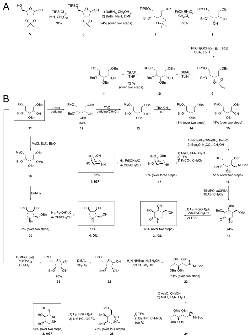
Fig. 2 Synthesis of galacto -configured azasugars. (A) Synthesis of key intermediate 11 from 2,3- O -isopropylidene-D-ribofuranose ( 5 ). (B) Synthesis of IGF, IGL, DIL and AGF from a common intermediate ( 11 ).
