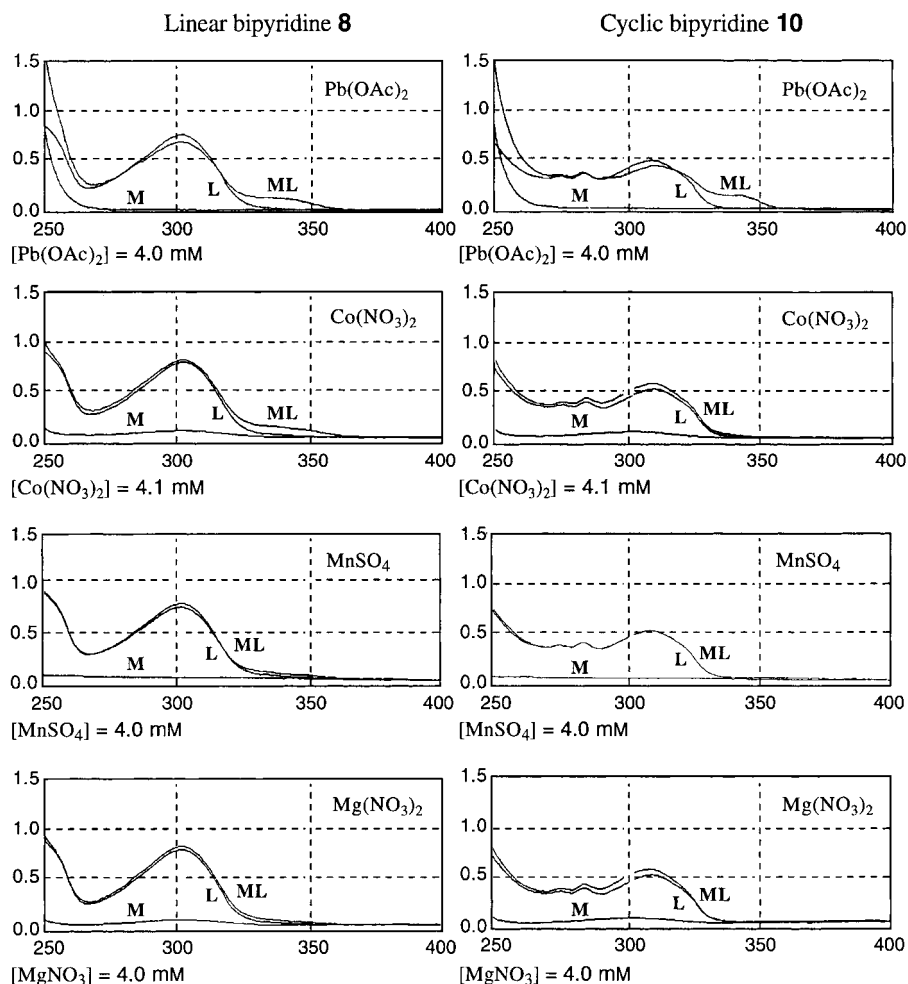
Fig. 5. UV Spectra of the mixtures of the linear bipyrindine 8 (left) and the cyclic bipyrindine 10 (right) with \text{Pb}(\text{OAc})_2 , \text{Co}(\text{NO}_3)_2 , \text{MnSO}_4 and \text{Mg}(\text{NO}_3)_2 . Extinction vs. wavelengths [nm]; in \text{H}_2\text{O} at 24^\circ . L: [ligand] = 0.04 mM; M: [metal salt] \approx 4 mM; ML: [ligand] = 0.04 mM and [metal salt] \approx 4 mM.
