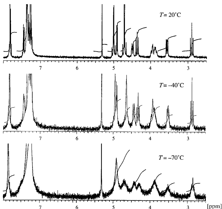
Fig. 2. ^1\text{H} -NMR Spectra (300 MHz, \text{CD}_2\text{Cl}_2 , 6.6 mm) of 5 at 20, -40 , and -70^\circ
