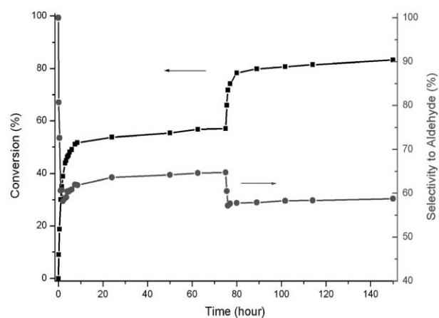
Fig. 2 The catalytic kinetics of benzyl alcohol oxidation with the additions of K 2 CO 3 . Catalysis conditions : 0.250 g of 2.5% 6.3 nm Au on TiO 2 ; 20 mL benzyl alcohol; 2 atm O 2 ; 0.280 g K 2 CO 3 were added at 0 and 75 h.
