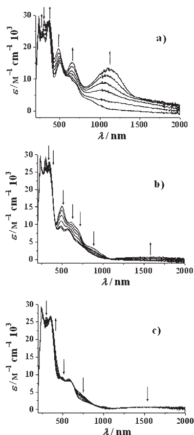
Figure 7. UV-visible-NIR spectroelectrochemistry for the conversions: a) 3^{2+} \rightarrow 3^{3+}/3^{4+} , b) 3^{2+} \rightarrow 3^{3+} , and c) 3^{3+} \rightarrow 3 in \text{CH}_3\text{CN}/0.1 \text{ M Bu}_4\text{NPF}_6 .
