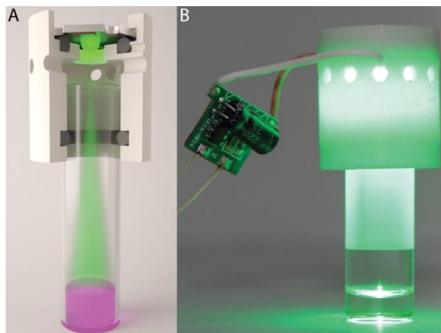
Figure 2. Computer model of designed photoreactor (A) and ready to use assembled photoreactor (B).
