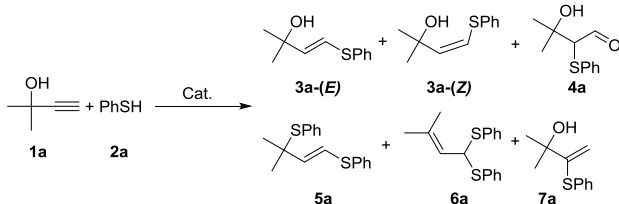
Scheme 2. Plausible products in the thiol–yne coupling process
