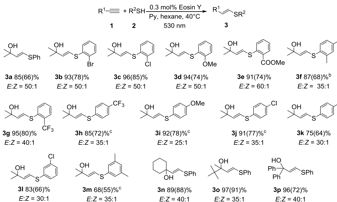
Scheme 3. The scope of the developed photocatalytic thiol–yne click reaction. a ( a Isolated yields are given in parentheses, reaction time – 3 h. b Reaction time - 10 h. c Reaction time - 20 h)
