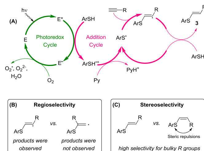
Scheme 4. The proposed mechanism (A) for the Eosin Y mediated thiol–yne photoredox coupling (Eosin Y is denoted with E), plausible origins of reaction regioselectivity (B) and stereoselectivity (C).
