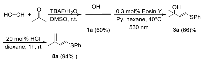
Scheme 5. The synthesis of diene 8a using the developed approach
