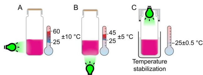
Figure 1. Comparison of the possible designs of the photoreactor: A – side irradiation (LED strip); B – bottom irradiation (LED matrix); C – developed design with temperature stabilization.
