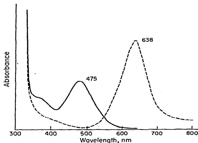
Fig. 4. Absorption spectra of N -[5-hydroxy-8-(4-nitrophenylazo)naphthyl]-1,3-benzenedisulfonamide; (—) acetone/HCl, \epsilon 11 000; (-----) acetone/NaOH, \epsilon 23 000.
