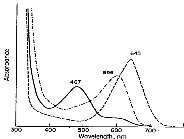
Fig. 3. Absorption spectra of N -[5-hydroxy-8-(4-dimesitylborylphenylazo)naphthyl]-1,3-benzenedisulfonamide; (—) acetone/HCl, \epsilon 4000; (---) acetone/NaOH, \epsilon 5000; (- - - -) sodium salt, \epsilon 9600.
