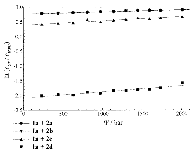
Figure 1. Dependence of the product ratio c_{cis}/c_{trans} on the El'yanov parameter \Psi for the cycloaddition reactions of phenylbutadiene 1a with the dicyanoethylenes 2a–d at 30 °C.
