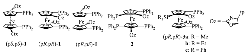
Fig. 1. Chiral ferrocene ligands derived from 1,1'-bis(oxazolinyl)ferrocene.
