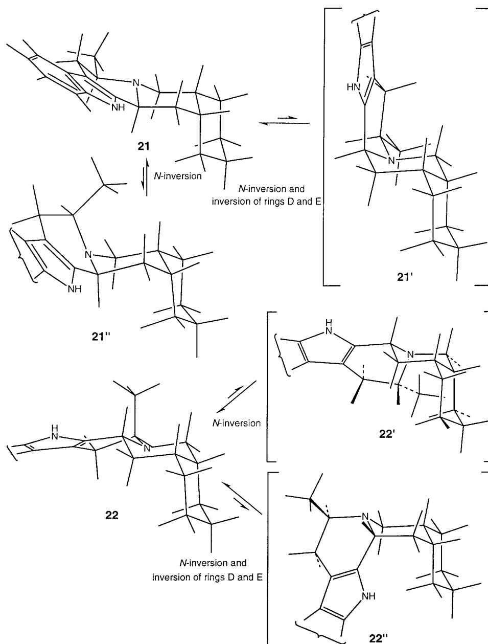
Fig. 2. Lowest-energy conformations of the four diastereoisomers of 5-methylyohimbane with cis-fused rings D and E as calculated by PM3. Unlabelled substituents represent H-atoms. Formulae in square brackets represent calculated, energetically higher lying conformers.
