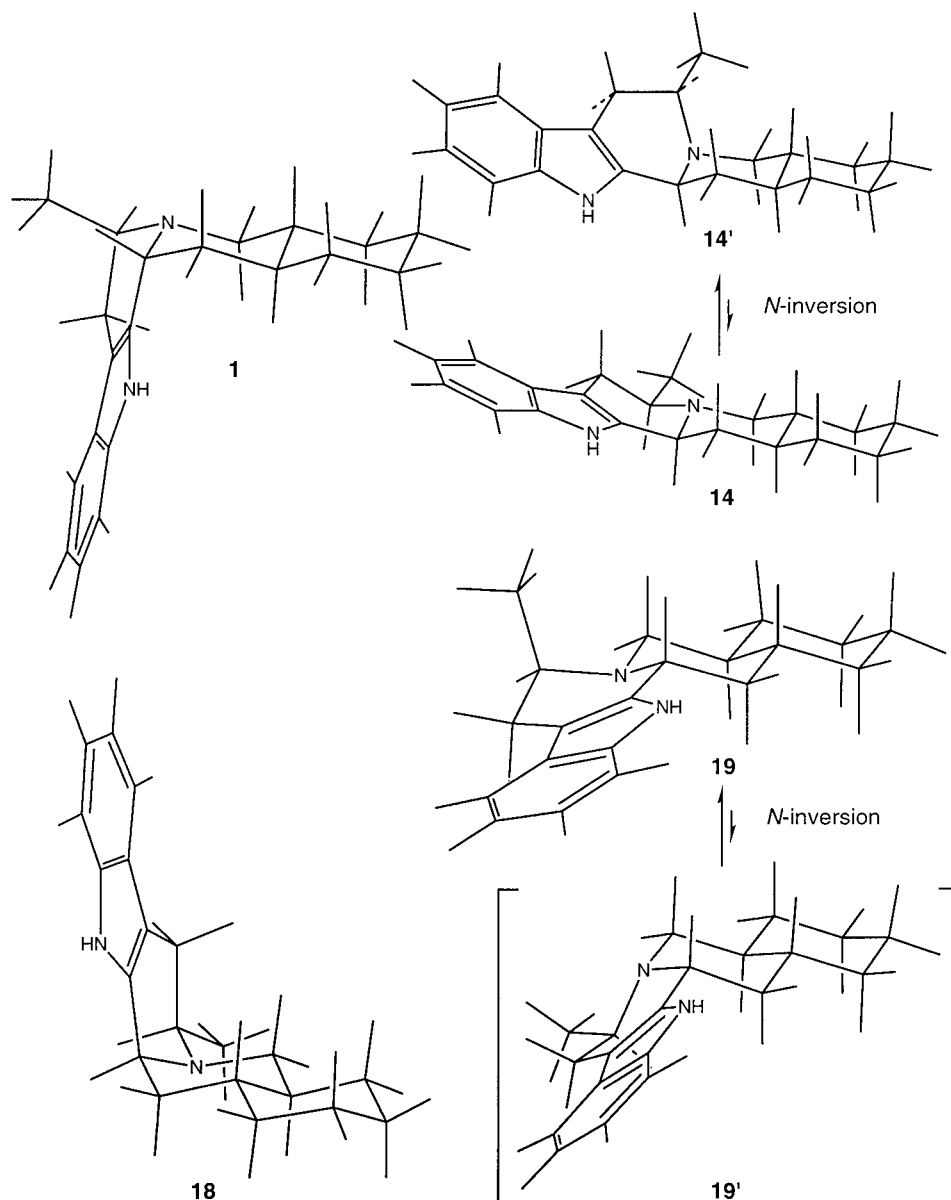
Fig. 1. Lowest-energy conformations of the four diastereoisomers of 5-methylyohimbane with trans-fused rings D and E as calculated by PM3. Unlabelled substituents represent H-atoms.
