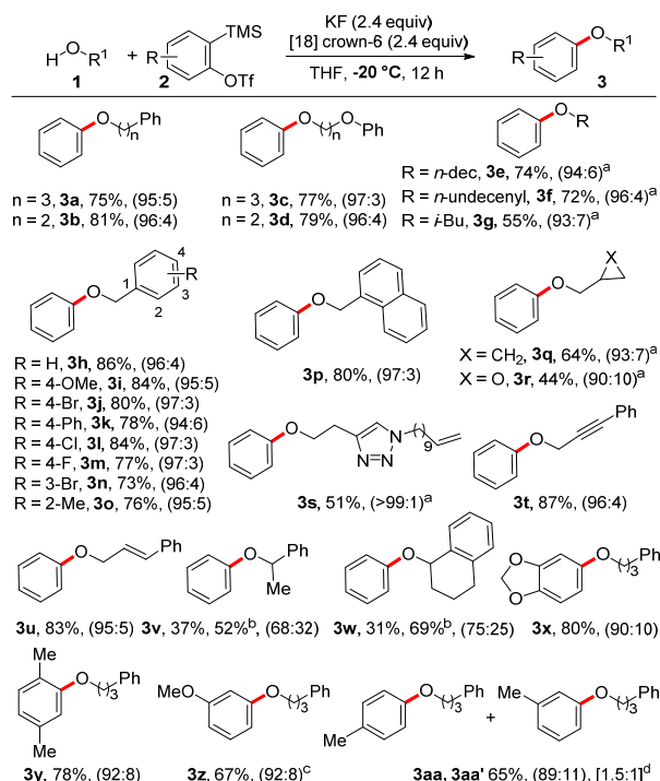
Scheme 1. Scope of the aryne insertion to O-H bond of alcohols. General conditions: 1 (0.5 mmol), 2 (0.6 mmol), KF (1.2 mmol), [18] crown-6 (1.2 mmol), THF (3.0 mL), -20 °C, 12 h. Yields of the isolated products are given. Selectivity ratio determined by GC analysis of crude reaction mixture is given in parentheses. a Reaction was run using 2.0 equiv of 2 , 4.0 equiv of KF and 4.0 equiv of [18]-crown-6. b Yield based on recovered 1 . c Reaction run on 0.25 mmol scale. d The regioisomer ratio determined by GC analysis.
