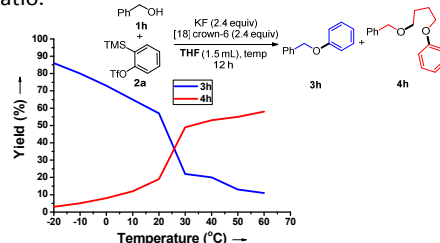
Figure 1. Variation of temperature on aryne reactions with benzyl alcohol
