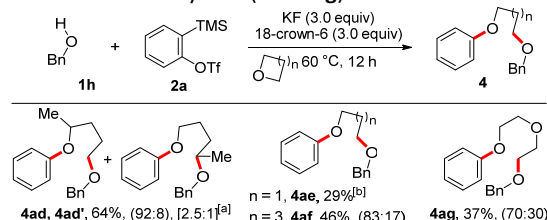
Scheme 3. Scope of the aryne MCCs with cyclic ethers. See the supporting information for details. Yields of the isolated products are given and selectivity ratio determined by GC analysis of crude reaction mixture is given in parentheses. a The regioisomer ratio determined by GC analysis. b NMR yield of the product given.
