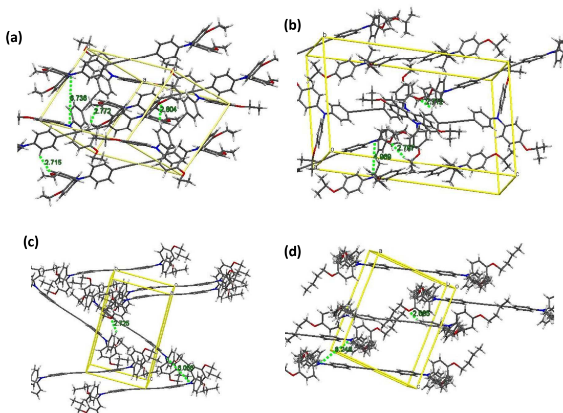
Figure 3. Crystal packing of all DATPA derivatives: (a) EtO-DATPA, (b) i PrO-DATPA, (c) n PrO-DATPA and (d) BuO-DATPA
