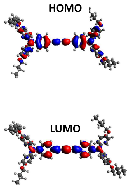
Figure 4. Molecular orbital distribution for BuO-DATPA at B3LYP/6-31G(d) level of theory.
