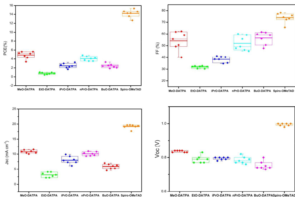
Figure 6. Solar cells parameters over 7 repeats for each HTM
