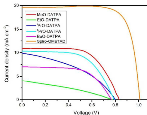
Figure 5. J-V curves (light and dark) of the champion PSCs with the DATPA series and Spiro-MeOTAD HTMs.
