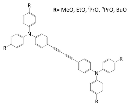
Figure 1. Chemical structure of HTMs used in this study. Each molecule is comprised of two bridged Ph 3 N moieties.
