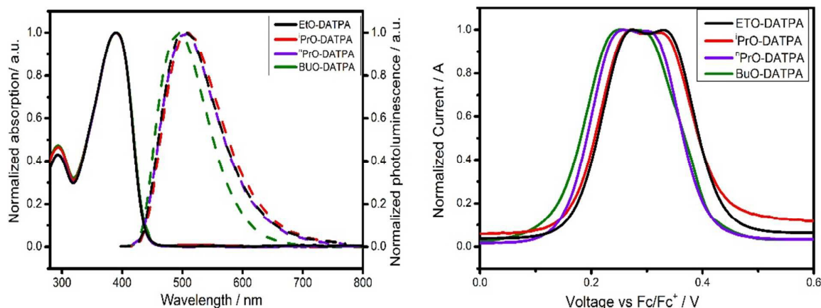
Figure 2. Left: Normalized UV-Vis absorption (solid line) and emission (dashed line) of each DATPA derivative. EtO-DATPA (black line), i PrO-DATPA (red line), n PrO-DATPA (purple line) and BuO-DATPA (green line). Right: Square-wave voltammetry of EtO-DATPA (black line), i PrO-DATPA (red line), n PrO-DATPA (purple line) BuO-DATPA (green line).
