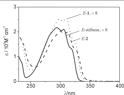
Fig. 1 Absorption spectra of E -stilbene (solid line), E -1 reference compound (dotted line) and E -2 dendrimer (dashed line) in acetonitrile solutions at 298 K.
