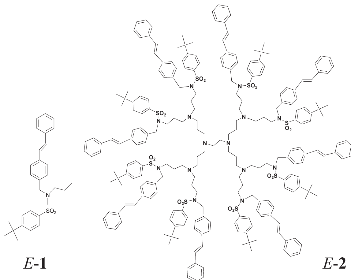
Scheme 2 Structure formulas of the E -form of 4- tert -butyl- N -propyl- N -(4-styryl-benzyl)benzenesulfonamide ( E -1), and of the second generation poly(propylene amine) dendrimer functionalized at the periphery with eight E -stilbene and eight 4- tert -butylbenzenesulfonyl units ( E -2).
