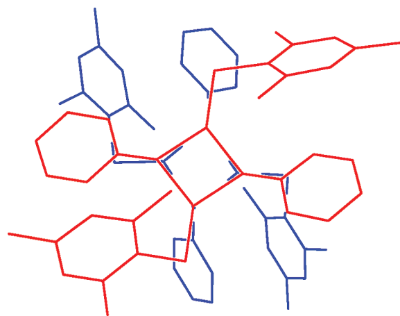
Figure 3. Projection along the pseudo- S_4 axis of the C_1 -symmetric structure of \text{Fe}_4(\text{NPh})_4(\text{SMes})_4 ( 3a ·1.5 \text{C}_6\text{H}_6 ), illustrating the idealized S_4 cluster symmetry and the disposition of the aryl ligand substituents. For clarity, top and bottom halves of the cluster are depicted in red and blue, respectively.
