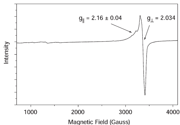
Figure 7. Perpendicular mode EPR spectrum of [\text{Fe}(\text{THF})_6][\text{Fe}_4(\text{N-}i\text{-p-Tol})_4(\text{SDMB})_3\text{N}(\text{SiMe}_3)_2]_2 ( [Fe(THF) 6 ][4] 2 ) (12 K, frozen toluene glass), with axial signal features indicated.
