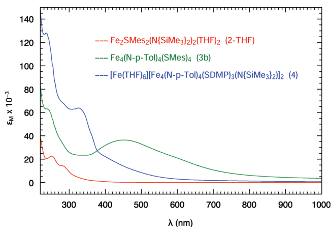
Figure 5. UV-visible absorption spectra of \text{Fe}_2(\text{SMes})_2(\text{N}\{\text{SiMe}_3\}_2)_2(\text{THF})_2 ( 2-THF ), \text{Fe}_4(\text{N-}i\text{-p-Tol})_4(\text{SMes})_4 ( 3b ), and [\text{Fe}(\text{THF})_6][\text{Fe}_4(\text{N-}i\text{-p-Tol})_4(\text{SDMB})_3\text{N}(\text{SiMe}_3)_2]_2 ( [Fe(THF) 6 ][4] 2 ) in THF. The spectrum of 2-THF (1.0 mM) cannot be associated definitively with the solid-state structure because of possible speciation in solution. The molar absorptivity of [Fe(THF) 6 ][4] 2 is normalized per cubane cluster.
