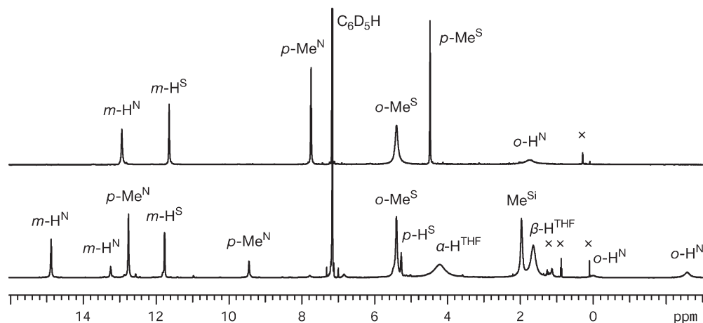
Figure 4. ^1\text{H} NMR spectra ( \text{C}_6\text{D}_6 , 500 MHz, 295 K) of \text{Fe}_4(\text{N-}i\text{-p-Tol})_4(\text{SMes})_4 ( 3b , top), and [\text{Fe}(\text{THF})_6][\text{Fe}_4(\text{N-}i\text{-p-Tol})_4(\text{SDMB})_3\text{N}(\text{SiMe}_3)_2]_2 ( [Fe(THF) 6 ][4] 2 , bottom). Resonances are labeled with superscripts indicating ligand type (N = imide, S = thiolate) and x = trace diamagnetic contaminants (solvent or silylmethyl-containing species).
