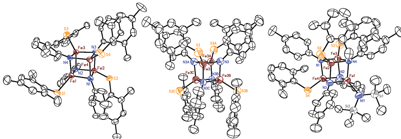
Figure 2. Structures of iron-arylimide cubane clusters \text{Fe}_4(\text{NPh})_4(\text{SMes})_4 ( 3a ·1.5 \text{C}_6\text{H}_6 , left), \text{Fe}_4(\text{N-}p\text{-Tol})_4(\text{SMes})_4 ( 3b ·0.5 \text{C}_6\text{H}_6 , tetragonal lattice, center), and [\text{Fe}_4(\text{N-}p\text{-Tol})_4(\text{SDMB})_3\text{N}(\text{SiMe}_3)_2]^- [\text{Fe}(\text{THF})_6][4]_2 \cdot 2\text{THF} , right), with thermal ellipsoids (50% probability level) and selected atom labels; hydrogen atoms are not shown. Two independent, complete clusters occur in the asymmetric unit of 3a ·1.5 \text{C}_6\text{H}_6 , of which one is shown above. In the asymmetric unit of tetragonal 3b ·0.5 \text{C}_6\text{H}_6 , three independent clusters exist, with two possessing crystallographic 4-fold rotoinversion symmetry and one having 2-fold rotational symmetry; one of the S_4 -symmetric clusters is depicted above, with labels ending in “A”, “B”, or “C” indicating atoms related by imposed symmetry. A second, monoclinic form of 3b is given as Supporting Information.
