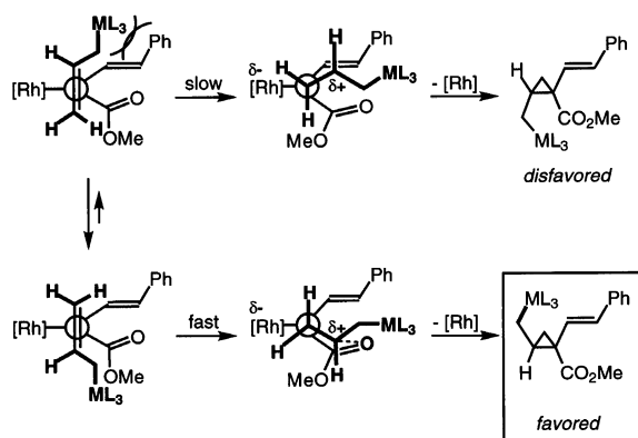
Fig. 5. Pathways for Rh_2(OAc)_4 -catalyzed cyclopropanation of allylmetals 6 with methyl 2-diazo-4-phenyl-3-butenate.
