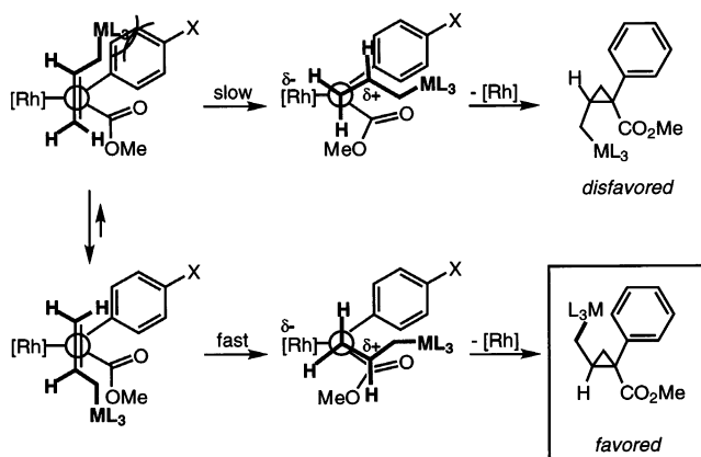
Fig. 6. Pathways for Rh_2(OAc)_4 -catalyzed cyclopropanation of allylmetals 6 with methyl 2-diazo-2-arylacrylates.
