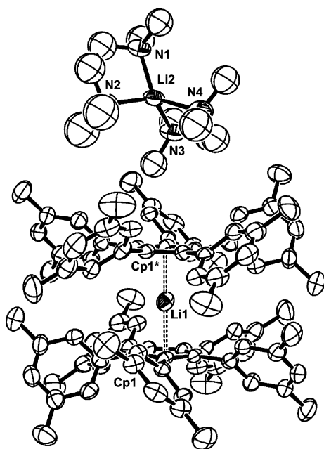
Fig. 5 Thermal ellipsoid view of [(\text{CpAr}^\#)_2\text{Li}][\text{Li}(\text{TMEDA})_2] ( 3a ) ( \text{Ar}^\# = 3,5\text{-Me}_2\text{C}_6\text{H}_3 ) drawn with 30% probability ellipsoids, giving the atom numbering scheme used in the tables. Only one of two independent molecules is shown. Cp1 is defined as the centroid arising from atoms C1–C5; Cp1* is defined as the centroid arising from atoms C1*–C5*. For the sake of clarity, only the centroid designations are given.
