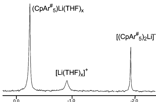
Fig. 6 194 MHz 7 Li NMR spectrum of {[(CpAr # ) 2 Li][Li(THF)](THF)} x ( 2a ) (Ar # = 3,5-Me 2 C 6 H 3 ) in C 6 D 6 at room temperature.
