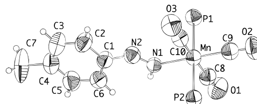
Figure 1. Perspective drawing of compound 1b , with anisotropic thermal displacement parameters represented as ellipsoids at the 40% level of probability. Phenyl and ethoxy groups have been omitted for clarity.
