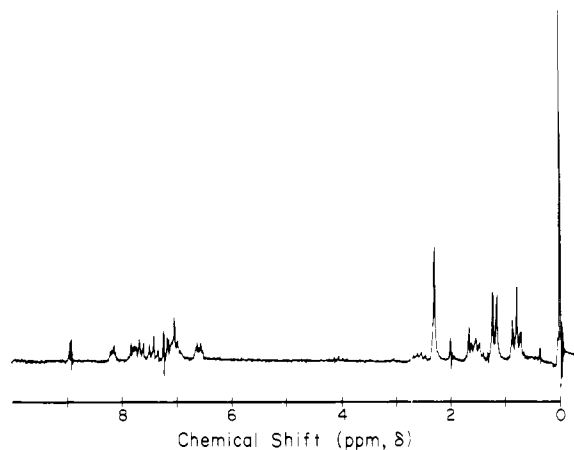
Figure 1. Proton NMR spectrum of (4'-MeL)CoL-LCo(4'-MeL)(ClO 4 ) 2 in CDCl 3 at 34 °C. Integration of the sec -butyl protons (0.8 and 1.1 ppm) and the methyl protons (2.3 ppm) provide evidence for describing the complex as binuclear.
