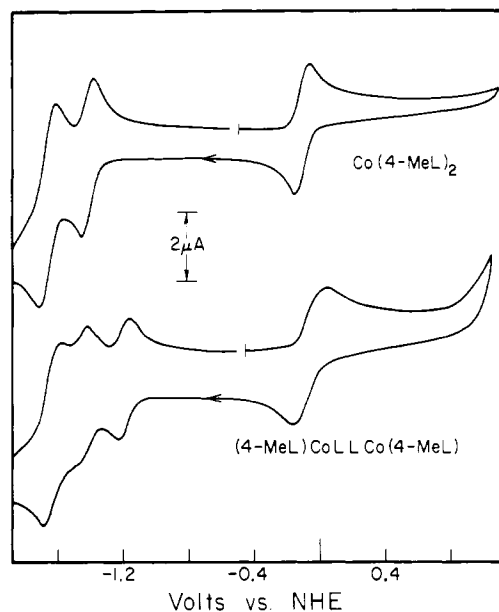
Figure 3. Cyclic voltammograms of DMF solutions: upper figure \text{Co}(4'\text{-MeL})_2 ; lower figure (4'\text{-MeL})\text{CoL}_2\text{Co}(4'\text{-MeL}) .
