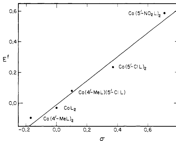
Figure 4. Half-wave potentials vs. \sigma_p for mononuclear \text{Co}(\text{II}) complexes containing various substituents on the isoindoline ligand.
