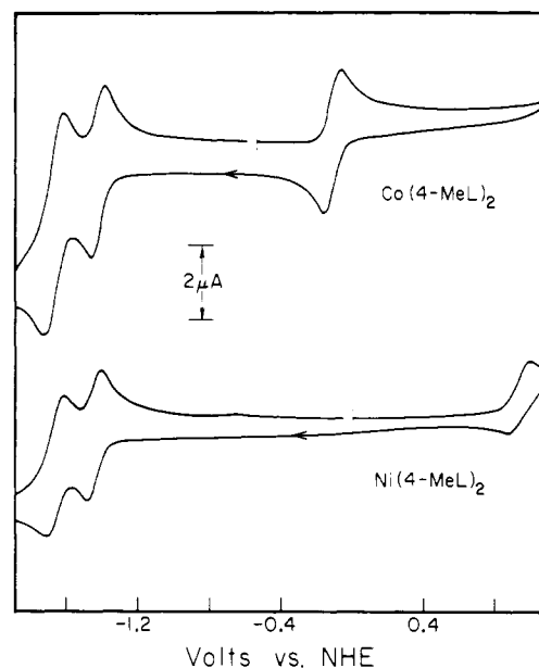
Figure 2. Cyclic voltammograms of DMF solutions: upper figure Co(4'-MeL) 2 ; lower figure Ni(4'-MeL) 2 .
