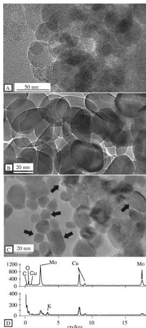
Figure 4. Solids from nanoscopic species in the mother liquor after 2–4 d. A) ppt1 . B) TEM at magnification 120k of polypent-Mo 2 by Method 2, dry preparation. C) TEM of polypent-Mo 2 by Method 3, wet preparation. D) Energy dispersive spectra of polypent-Mo 2 (top) and ppt1 (bottom). The Cu grid produced the Cu peaks.
