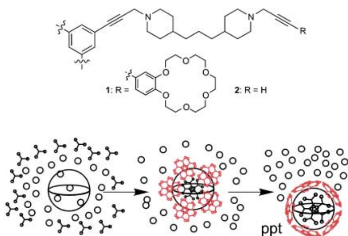
Figure 1. Top: tripodal molecules used to trap polypent-Mo 2 ; bottom: schematic representation of kinetic precipitation of polypent-Mo 2 . The circles represent solvent; the triangles represent tripodal molecules 1 ; and the large sphere represents nanoscale polypent-Mo 2 aqueous species. Kinetic solution state structure is preserved in the solid.
