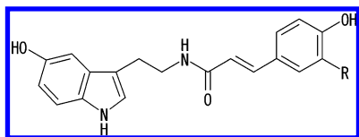
Figure 1. Structure of serotonin derivatives CS, R=H; FS, R=OCH 3 .
