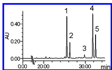
Figure 3. HPLC-UV chromatogram of the ethyl acetate fraction of the ethanolic extract of defatted safflower seeds (SSE). Detection = 290 nm. Peaks: 1, CS-monoglucoside; 2, FS-monoglucoside; 3, 2-hydroxyarctiin; 4, CS; 5, FS.
