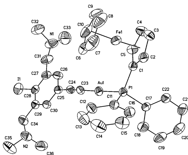
Figure 3. ORTEP (50% ellipsoid probability level) of 3c with the atom-numbering scheme (the hydrogen atoms are omitted for clarity).
