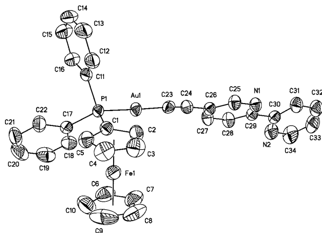
Figure 1. ORTEP (50% ellipsoid probability level) of 3a with the atom-numbering scheme (the hydrogen atoms and one molecule of dichloromethane are omitted for clarity).
