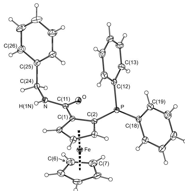
Figure 1. PLATON plot of the molecular structure of (S p )-2. Displacement ellipsoids are shown at the 30% probability level. Only labels for the pivotal and their adjacent carbon atoms with the consecutively numbered rings are shown.
