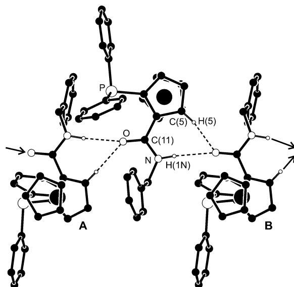
Figure 2. Section of the hydrogen-bonded assembly in the structure of ( S p )-2 showing hydrogen bonds as dashed lines (only hydrogen-bonded H atoms are shown). Symmetry operations: A: -x, y + 1/2, 1/2 - z ; B: -x, y - 1/2, 1/2 - z . Selected parameters: N···O = 3.284(2) Å, angle at H(1N) = 170°; C(5)···O = 3.150(2) Å, angle at H(5) = 151°.
