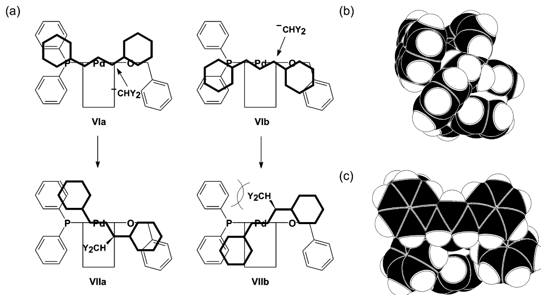
Scheme 5. (a) Idealized Depiction of the Plausible Reaction Intermediates VI and VII ( Y = \text{CO}_2\text{Me} ); (b,c) Space-Filling Model of the Cation in ( S_p )- 8 as Viewed (b) along the C(33)–C(31) Line (i.e., from the benzyl group) and (c) Perpendicular to the \eta^3 -Allyl Moiety
