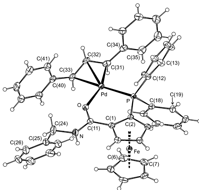
Figure 3. PLATON plot of the cation in the structure of ( S p )-8·Me 2 CO. Displacement ellipsoids correspond to 30% probability. The ring atoms are numbered consecutively and, hence, the labels of only the pivotal and their adjacent carbon atoms are shown to avoid complicating the figure.
