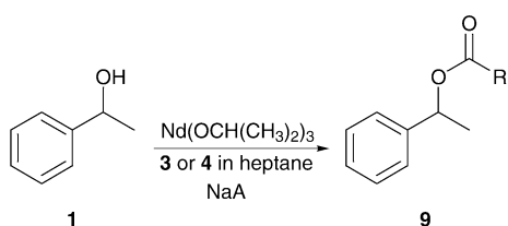
Scheme 4 \text{Nd}(\text{OCH}(\text{CH}_3)_2)_3 catalysed acylation with 3 and 4 .
