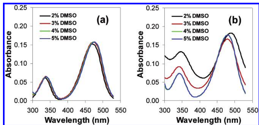
Figure 1. UV spectra of (a) monomer 10 and (b) heptamer 13 in DMSO/ \text{CCl}_4 mixtures. [\mathbf{10}] = [\mathbf{13}] = 10 \mu\text{M} .
