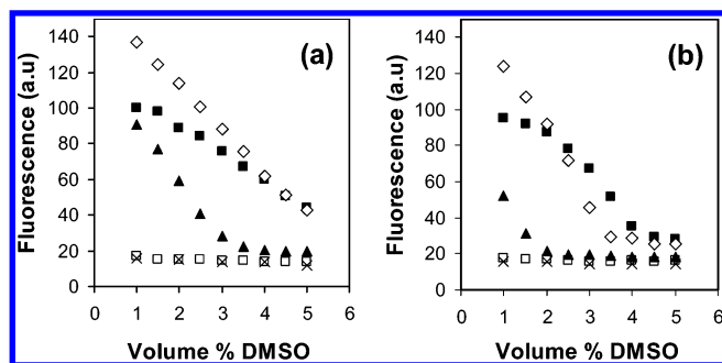
Figure 8. Maximum emission intensity of the acceptor in PDA 16 (▲), HXDA 17 (◇), HPDA 18 (■), MA 19 (□), and a 1:1 mixture (19 + 20) of MA and MD (×) as a function of the volume percentage of DMSO in (a) ethyl acetate/hexane (1/2) and (b) ethyl acetate/hexane (1/1).
