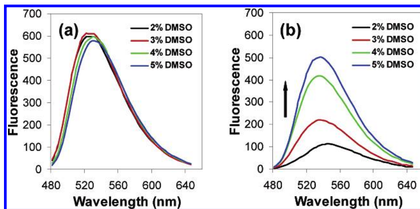
Figure 3. Fluorescence spectra of (a) monomer 10 and (b) heptamer 13 in DMSO/CCl 4 mixtures. [ 10 ] = [ 13 ] = 10 \mu M.
