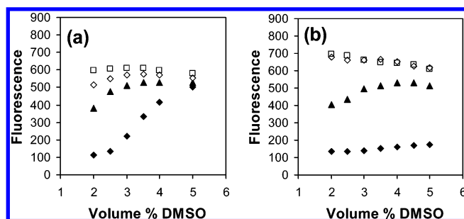
Figure 4. Maximum fluorescence intensity of monomer 10 ( \square ), trimer 11 ( \diamond ), pentamer 12 ( \blacktriangle ), and heptamer 13 ( \blacklozenge ) as a function of DMSO in (a) CCl 4 and (b) ethyl acetate/hexane = 1/2. [Oligomer] = 10 \mu M.
