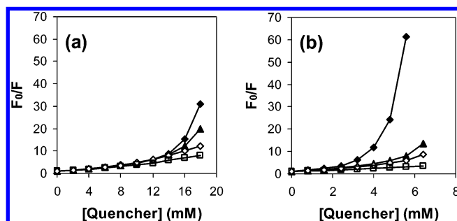
Figure 5. Quenching of monomer 10 ( \square ), trimer 11 ( \diamond ), pentamer 12 ( \blacktriangle ), and heptamer 13 ( \blacklozenge ) by hydrophilic quencher 14 in (a) 5% DMSO/CCl 4 and (b) 2% MeOH/CCl 4 . [Oligomer] = 12.5 \mu M.
