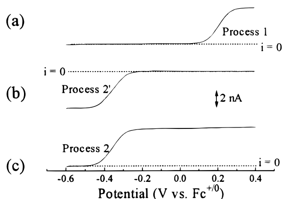
Figure 3. Microdisk near steady-state voltammograms obtained at -40^{\circ}\text{C} with a 25\text{ }\mu\text{m} diameter platinum electrode (scan rate 10\text{ mV s}^{-1} ) from an initially 1.0\text{ mM} solution of 1A in dichloromethane ( 0.1\text{ M} \text{Bu}_4\text{NPF}_6 ) (a) before electrolysis, (b) after electrolysis at +0.25\text{ V} , and (c) after reduction of the solution formed in (b) at -0.55\text{ V} .
