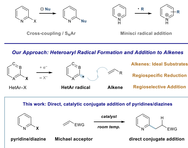
Figure 1. General Strategies for the synthesis of complex heteroarenes
