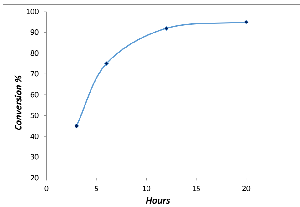
Figure 3. Conversion of 3a vs time in the Henry reaction catalysed by 8b-BF 4 / \text{Cs}_2\text{CO}_3 in \text{CH}_2\text{Cl}_2 at 30 °C.
