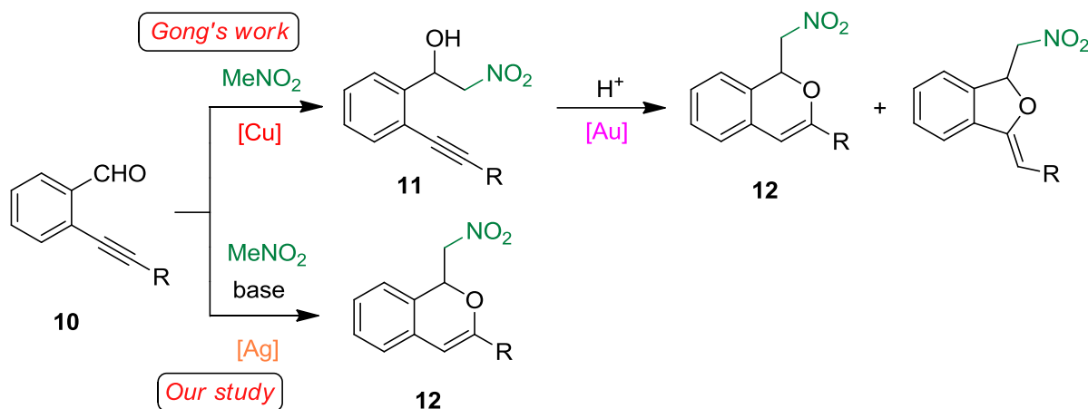
Scheme 5. Alternative domino silver(I) catalysed synthesis of 1-isochromenes.
