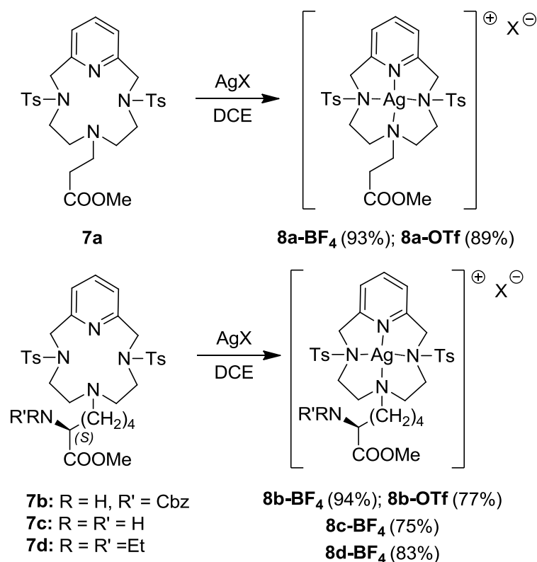
Scheme 3. Synthesis of silver(I) complexes 8a-d .
