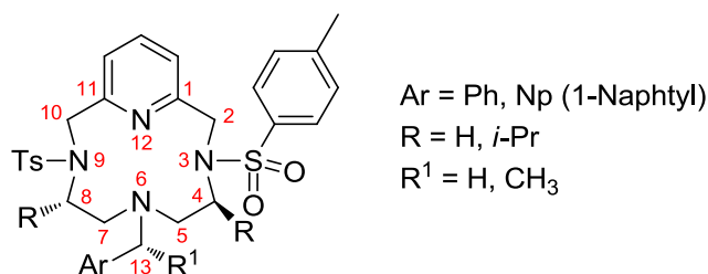
Figure 1. Pyridine-containing ligand (Pc-L*) and numbering scheme adopted.
