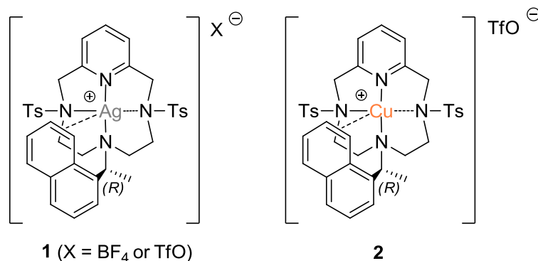
Figure 2. Silver ( 1 ) and copper ( 2 ) PcL-complexes tested in the model Henry reaction.
