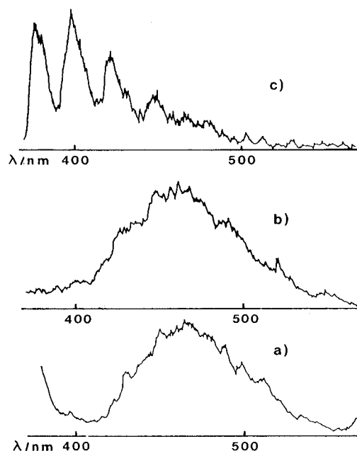
Figure 4. Dispersed fluorescence spectra excited at (a) 370.70 nm (26 976 cm -1 ), (b) 359.40 nm (27 824 cm -1 ), and (c) 355.10 nm (28 162 cm -1 ). The excitation bands are indicated by arrows in Figure 3.
