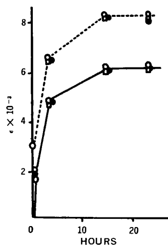
Figure 6 —Effect of ferric chloride and allyl alcohol on the reaction of I with hydrogen peroxide at pH 7.9. Compound I-HCl ( 7.6 \times 10^{-4} M ) was treated with 0.025 M hydrogen peroxide in 0.1 M phosphate buffer (pH 7.9) at room temperature. Absorbance at 315 nm when diluted with 0.1 N NaOH and that at 285 nm when diluted with 0.1 N HCl were measured. Key: —, 315 nm; ---, 285 nm; ○, with none; ●, with 5 \times 10^{-5} M ferric chloride; and □, with 5 \times 10^{-2} M allyl alcohol.
