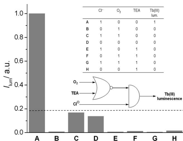
Fig. 3 Normalised Tb(III) luminescence intensities of a 1:1 mixture with 1 (75 \mu M, MeCN) at \lambda_{\text{obs}} = 544 nm with different chemical inputs [Cl - : 150 \mu M; O 2 : 1.9 mM (air-equilibrated); TEA: 75 \mu M]. The dashed line marks the threshold. The insets show the logic table and the respective symbolic representation of the EnNOR function.
