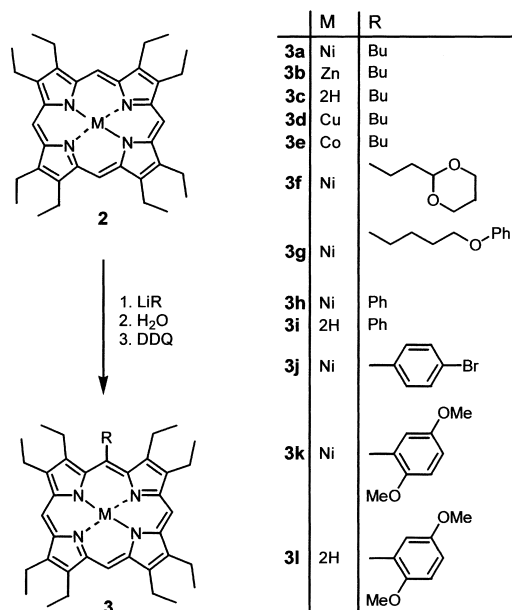
Scheme 1. meso Monofunctionalization of (metallo)octaethylporphyrins.
