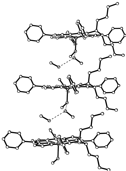
Figure 9. View of the molecular stacks formed by 17(MeOH) in the crystal. Dashed lines indicate hydrogen bonding; hydrogen atoms have been omitted for clarity. Selected bond lengths and angles: Zn–N(21) 2.112(4) \text{ \AA} , Zn–N(22) 2.056(4) \text{ \AA} , Zn–N(23) 2.099(4) \text{ \AA} , Zn–N(24) 2.043(4) \text{ \AA} , Zn–O(1A) 2.116(3) \text{ \AA} , C(2)–C(3) 1.515(6) \text{ \AA} , C(1)–C(2)–C(3) 101.2(4)^\circ , C(3)–C(2)–C(21) 112.1(4)^\circ , C(1)–C(2)–C(21) 110.5(4)^\circ , C(2)–C(3)–C(4) 102.2(4)^\circ .
