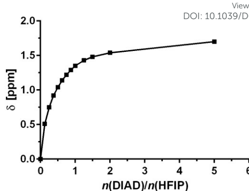
Figure 1 NMR titration curve of HFIP with DIAD 5b .
