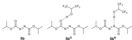
Figure 2 DIAD 5b , DIAD-HFIP complex H-bonded through a carbonyl oxygen atom 5b O and DIAD-HFIP complex H-bonded through a nitrogen atom 5b N .
