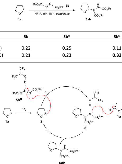
Scheme 5 Proposed mechanism.
