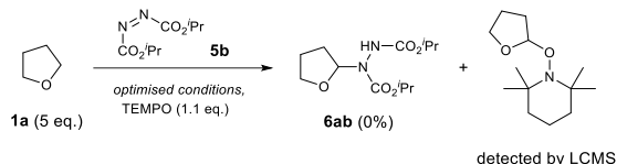
Scheme 4 TEMPO trapping experiment.
