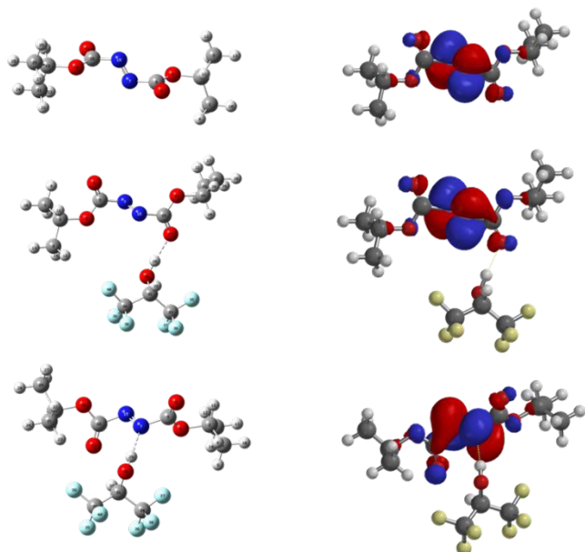
Figure 3 (Left) Optimised geometry of 5b , 5b O and 5b N at M06-2X/6-311++G(d,p) level. (Right) Corresponding calculated LUMO.
