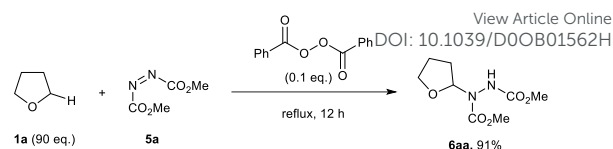
Scheme 2 Previously reported peroxide-initiated synthesis of adduct 6aa requiring a vast excess of THF 1a .
