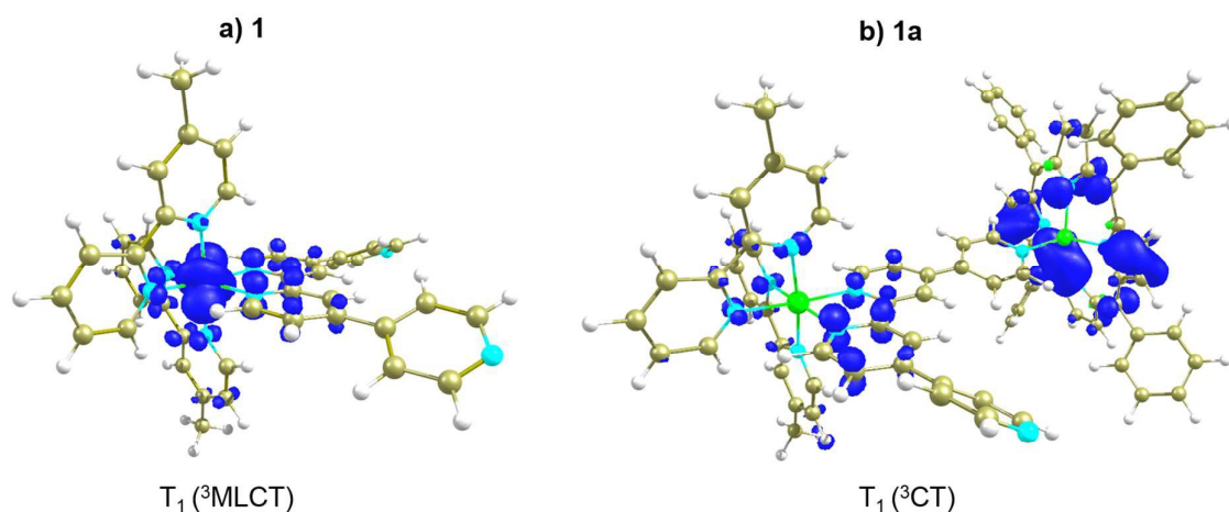
Figure 6. Spin-density distributions [B3LYP/6-31G(d) – ecp-28-mwb for Ru] at the optimized geometry of the lowest triplet excited state of 1 (a) and 1a (b).
