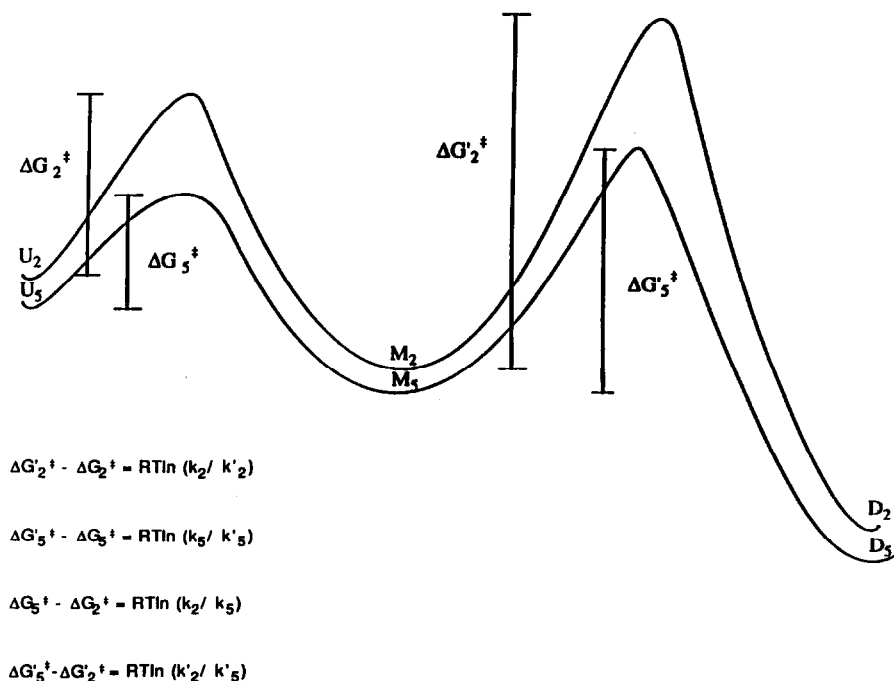
Fig. 5. Energy diagram illustrating the ground states and transition states of 1,2-diphenyltetramethyldisilane and 1,5-diphenyldecamethylpentasilane and the corresponding monofunctionalized products.
