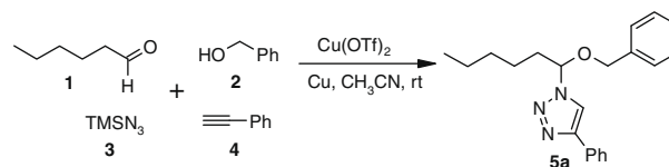
Scheme 1. Preparation of \alpha -alkoxytriazole 5a .
