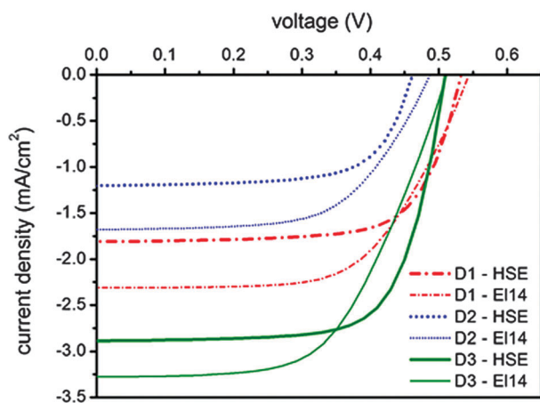
Fig. 5 Current-voltage curves for the DSSCs sensitized by the ruthenium-based dyes under 1 Sun illumination, AM 1.5. Two different iodide/triiodide electrolytes were used, a commercially available one (HSE, Dyesol) and another developed in-house (labeled E114).
