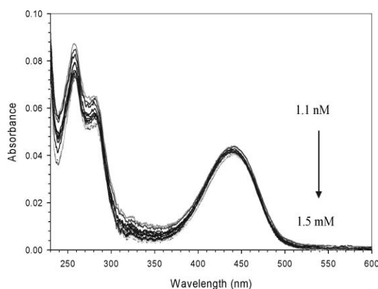
Fig. 5 Absorption spectra response of 1 in the presence of increasing concentration of Zn(II) ( cf. Fig. 4) in HEPES buffer at pH 7.4.
