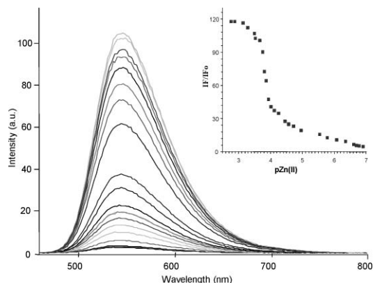
Fig. 4 Changes in the fluorescence emission spectra of 1 (1 \mu\text{M} ) upon addition of Zn(II) upon excitation at 422 nm, at pH 7.4. [Zn(II)]: 1.2 nM–1.5 mM. Insert : The changes at 550 nm as a function of -\log[\text{Zn(II)}] , pZn.
