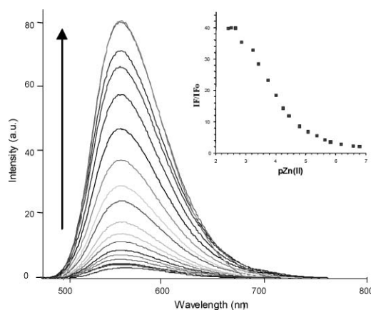
Fig. 6 Changes in the fluorescence emission spectra of 2 ( 1 \times 10^{-6} \text{ M} ) upon addition of Zn(II) upon excitation at 455 nm, at pH 7.4. [Zn(II)] are the same as in Fig. 4. Insert : The changes at 554 nm as a function of pZn ( = -\log[\text{Zn(II)}] ).
