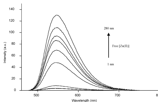
Fig. 8 Changes in the fluorescence emission spectra of 1 upon addition of Zn(II) upon excitation at 455 nm, at pH 7.4 (20 mM HEPES) and 135 mM KCl and 1.1 mM EGTA.
