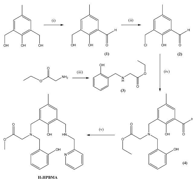
Scheme 1 Synthesis of \text{H}_2\text{HPBMA} ; (i) \text{MnO}_2 ; (ii) conc. \text{HCl} ; (iii) salicylaldehyde- \text{NaBH}_4 ; (iv) (2) + (3); (v) (4) + 2-aminomethylpyridine, \text{NaBH}_4 , methanol.
