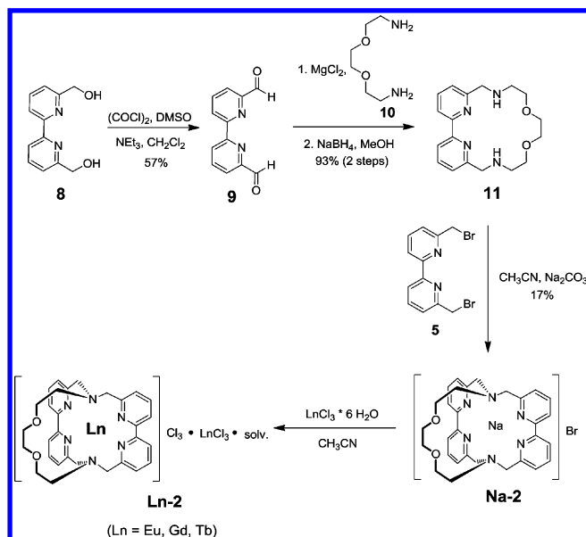
Scheme 3. Synthesis of the Lanthanoid Cryptates Ln-2
