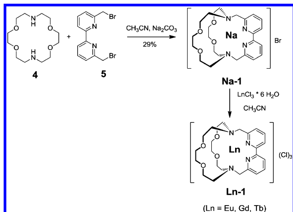
Scheme 1. Synthesis of the Lanthanoid Cryptates Ln-1
