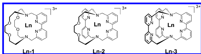
Figure 1. Known 2,2'-bipyridine-based lanthanoid cryptates Ln-1 and Ln-3 and new lanthanoid cryptate Ln-2 with an intermediate number of bipyridine arms.
