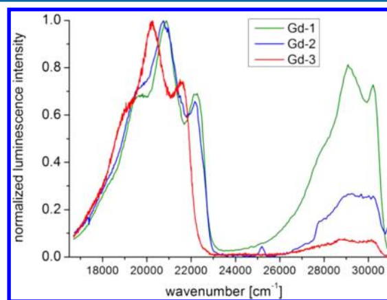
Figure 7. Low-temperature (77 K) steady-state emission spectra of Gd-1, Gd-2, and Gd-3 ( \lambda_{\text{exc}} = 304 nm, MeOH/EtOH, 1:1, v/v).
