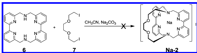
Scheme 2. Attempted Synthesis of the Sodium Cryptate Na-2
