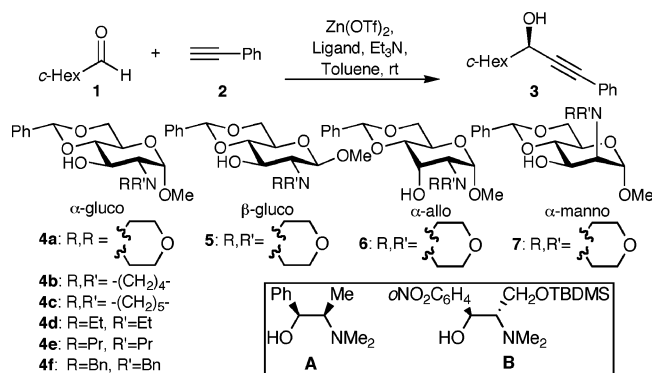
Scheme 1. Stereochemically and Functionally Diverse Family of Ligands Tested in Zn(OTf) 2 -Promoted Alkynylation
