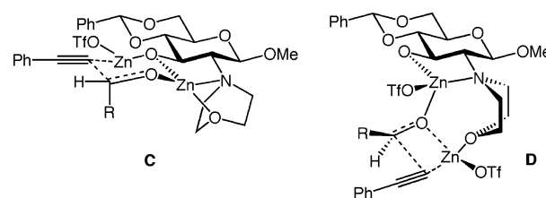
Figure 1. Proposed transition states.
