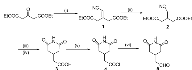
Fig. 2. The Synthesis of the Common Intermediate 3-Glutarimidylacetaldehyde
