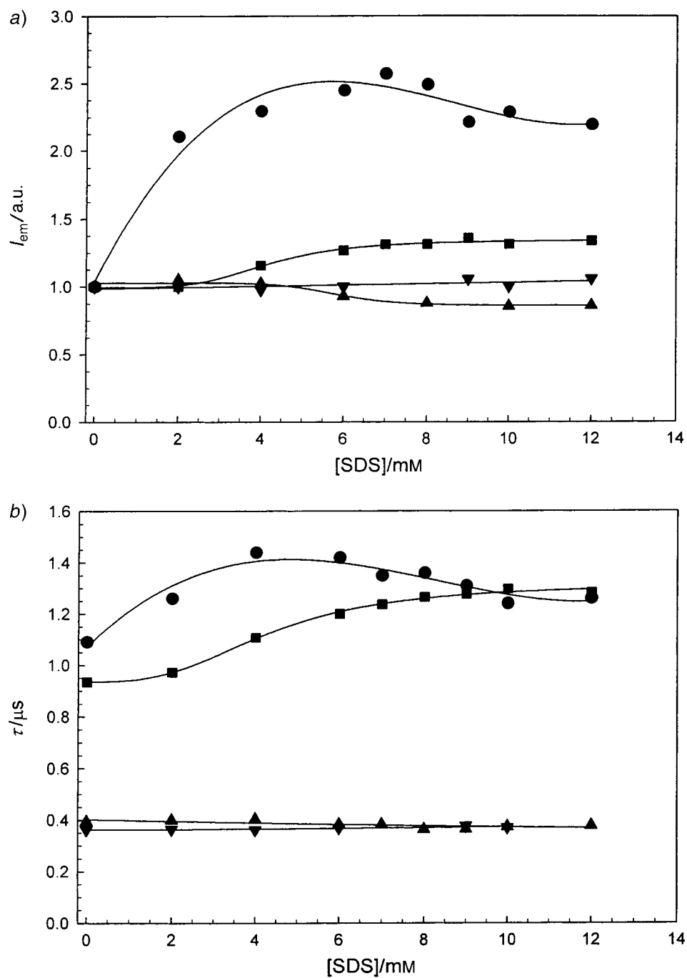
Fig. 3. a) Normalized emission intensity and b) lifetimes of the [RuL_2L']^{2-} complexes ( 1\ \mu M in air-equilibrated water) in the presence of SDS: [Ru(pbbs)_2(pta)]^{2-} ( 5a ; ●), [Ru(pbbs)_2(paa)]^{2-} ( 5b ; ■), [Ru(bpds)_2(pta)]^{2-} ( 6a ; ▲), and [Ru(bpds)_2(paa)]^{2-} ( 6b ; ▼)
