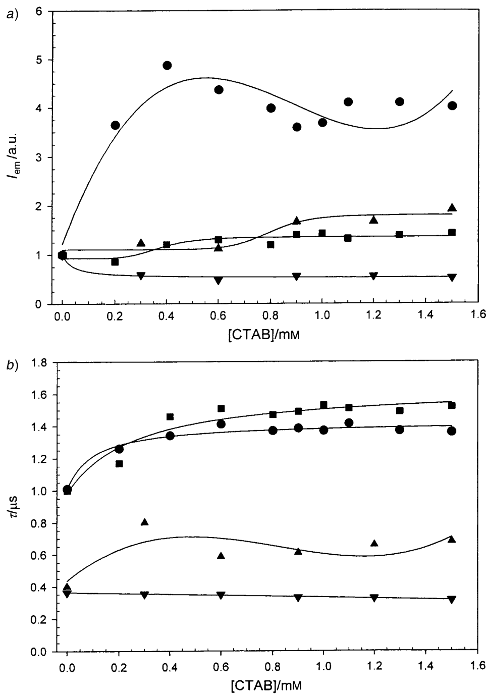
Fig. 4. a) Normalized emission intensity and b) lifetimes of the [RuL_2L']^{2-} complexes ( 0.3 \mu M in air-equilibrated water) in the presence of CTAB: [Ru(pbbs)_2(pta)]^{2-} ( 5a ; ●), [Ru(pbbs)_2(paa)]^{2-} ( 5b ; ■), [Ru(bpds)_2(pta)]^{2-} ( 6a ; ▲), [Ru(bpds)_2(paa)]^{2-} ( 6b ; ▼)
