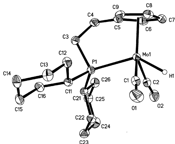
Figure 2. Molecular structure of \text{HMo(CO)}_2[\eta^5:\eta^1\text{-C}_5\text{H}_4\text{-(CH}_2)_2\text{PCy}_2] , 2Cy . Thermal ellipsoids were drawn at the 50% probability level. All hydrogens except H(1) were removed for clarity.
