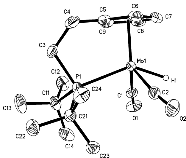
Figure 3. Molecular structure of \text{HMo(CO)}_2[\eta^5:\eta^1\text{-C}_5\text{H}_4\text{-(CH}_2)_2\text{P}^t\text{Bu}_2] , 2 t Bu . Thermal ellipsoids were drawn at the 50% probability level. All hydrogens except H(1) were removed for clarity.
