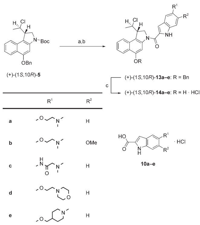
Scheme 4. Synthesis of seco-drug hydrochlorides (+)-(1S,10R)-14a-e: a) 4 M HCl/EtOAc, RT, 3–3.5 h; b) 10a-e , EDC·HCl, DMF, RT, 19–24 h; c) 4 M HCl/EtOAc, RT, 2 h, then Pd/C/NH 4 HCO 2 , THF, 40 °C, 20–120 min; yields from (+)- 5 : (+)- 14a : 65 %, (+)- 14b : 57 %, (+)- 14c : 66 %, (+)- 14d : 69 %, (+)- 14e : 62 %.
