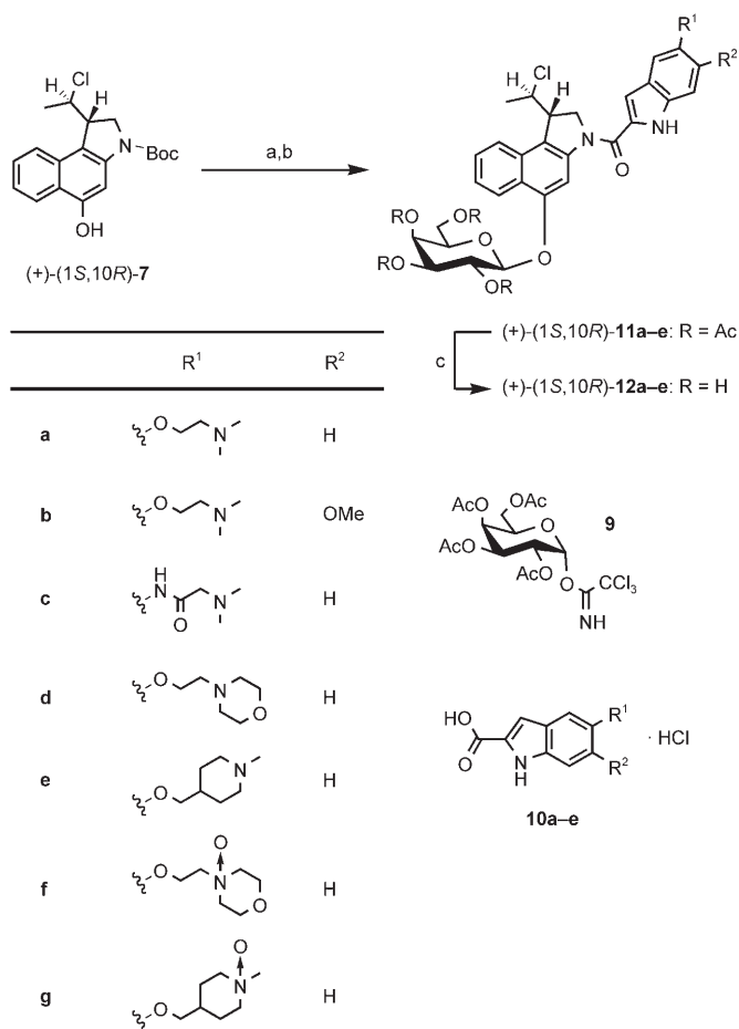
Scheme 3. Synthesis of β-D-galactosidic prodrugs (+)-(1 S ,10 R )- 12a–e : a) 9 , BF 3 ·OEt 2 , CH 2 Cl 2 , 4 Å MS, –10°C → RT, 9 h; b) 10a–c , EDC·HCl, DMF, RT, 20–22 h; 10d,e , EDC·HCl, DMF, RT, 20–22 h, then PtO 2 ·H 2 O/H 2 , EtOH, RT, 5–16 h; c) NaOMe/MeOH, RT, 20–120 min; yields from (+)- 7 : (+)- 12a : 46%, (+)- 12b : 43%, (+)- 12c : 39%, (+)- 12d : 29%, (+)- 12e : 36%.
