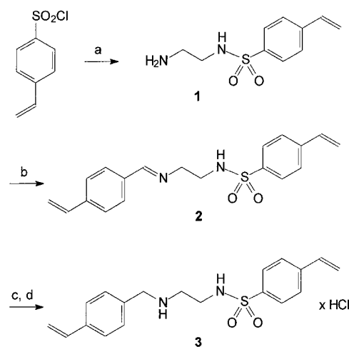
Scheme 3. a) H 2 NCH 2 CH 2 NH 2 , CH 2 Cl 2 ; b) 4-vinylbenzaldehyde, 4 Å, CH 2 Cl 2 ; c) NaBH 4 , MeOH; d) HCl/Et 2 O.
