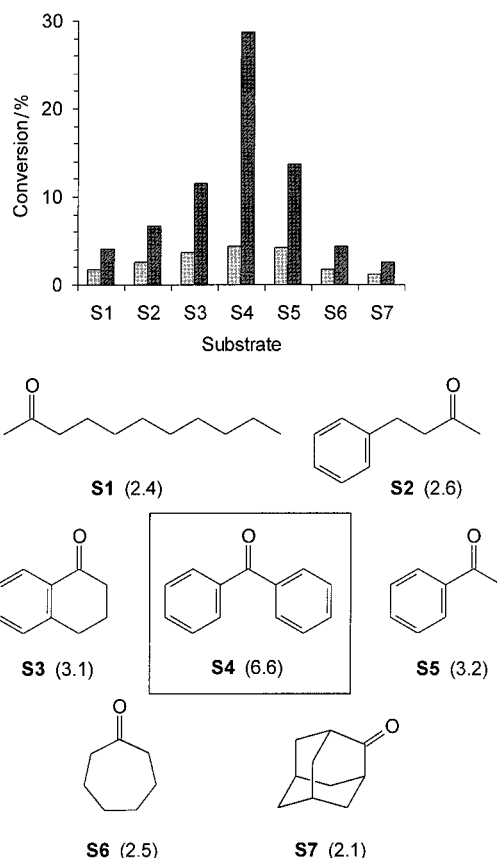
Figure 4. Transfer hydrogenation of a mixture of seven different ketones ( S1 – S7 ) in the presence of catalyst P8 or P6 . Product distribution after 20 min reveals that the MIP catalyst P8 (dark grey) is significantly more active than the control catalyst P6 (light grey). Furthermore, P8 shows a pronounced selectivity for benzophenone. The values for the relative increase in yields are reported below.
