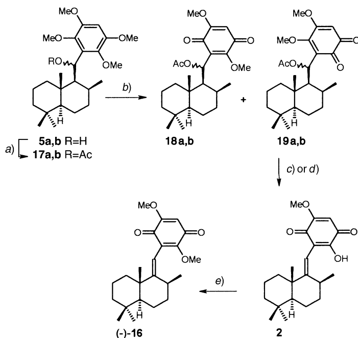
Scheme 10
