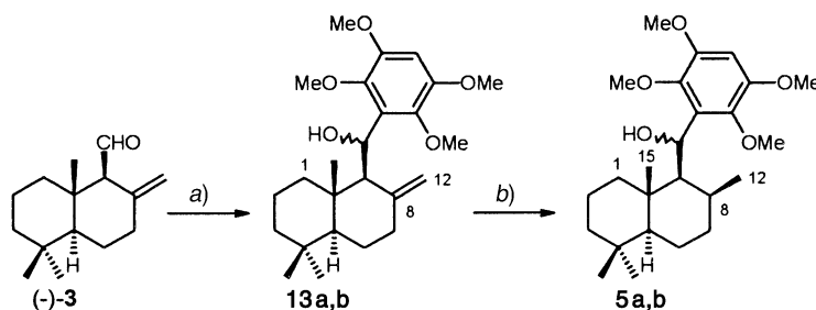
Scheme 7
