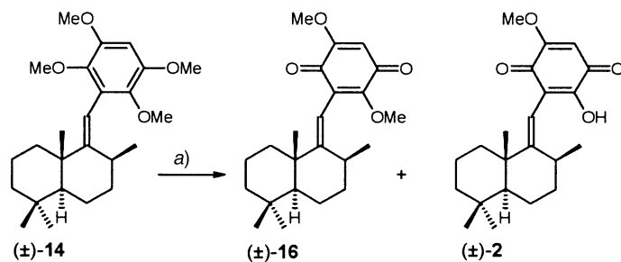
Scheme 9
