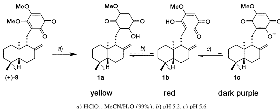
Scheme 4
