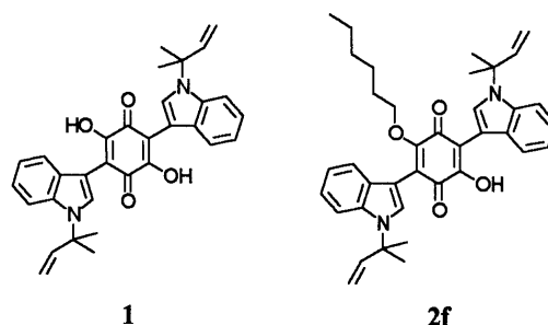
Fig. 1. Chemical Structures of Asterriquinone ( 1 ) and Asterriquinone Monoethyl Ether ( 2f )
