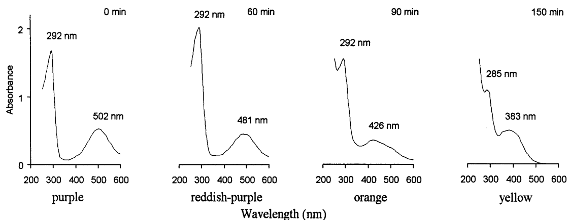
Fig. 2. The UV Spectrophotometric Course of the Reaction Mixture
