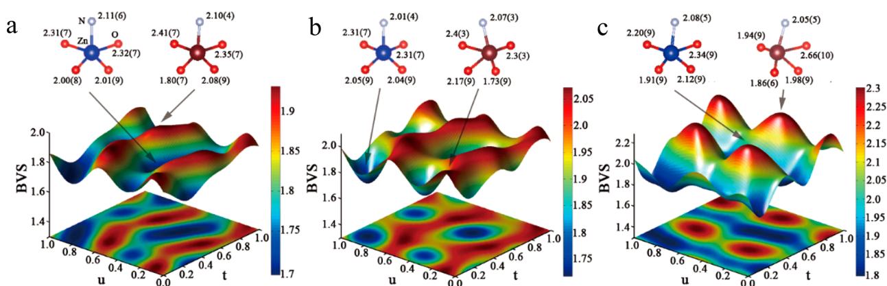
Figure 3. Maps of the bond valence sum (BVS) analyses of the oxidation state of Zn(II) centers as a function of the modulation vector u and t in (a) MFM-520, (b) MFM-520- \text{CO}_2 , and (c) MFM-520- \text{SO}_2 . The coordination geometries of the [\text{ZnO}_4\text{N}] polyhedra for the lowest and highest (highlighted in blue and brown, respectively) BVS analysis maps for MFM-520, MFM-520- \text{CO}_2 , and MFM-520- \text{SO}_2 are illustrated above the contour maps. Bond distances are in Å. BVS parameters R_{ij}(\text{Zn}-\text{O}) , b_0(\text{Zn}-\text{O}) , R_{ij}(\text{Zn}-\text{N}) , and b_0(\text{Zn}-\text{N}) are 1.704, 0.37, 1.72, and 0.37 Å, respectively. MFM-520- \text{H}_2\text{O} has a periodic structure and shows no modulation by BVS analysis; the formal oxidation state of all Zn(II) centers in MFM-520- \text{H}_2\text{O} is 1.974(14).
