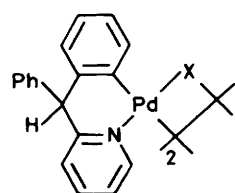
(1) X = MeCO 2 −
